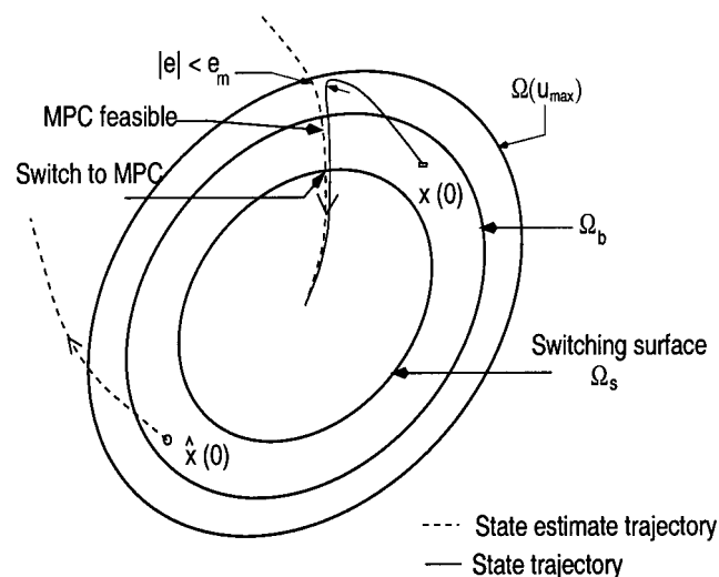
Figure 4. Evolution of the closed-loop system under the controller switching strategy proposed in Theorem 1.
